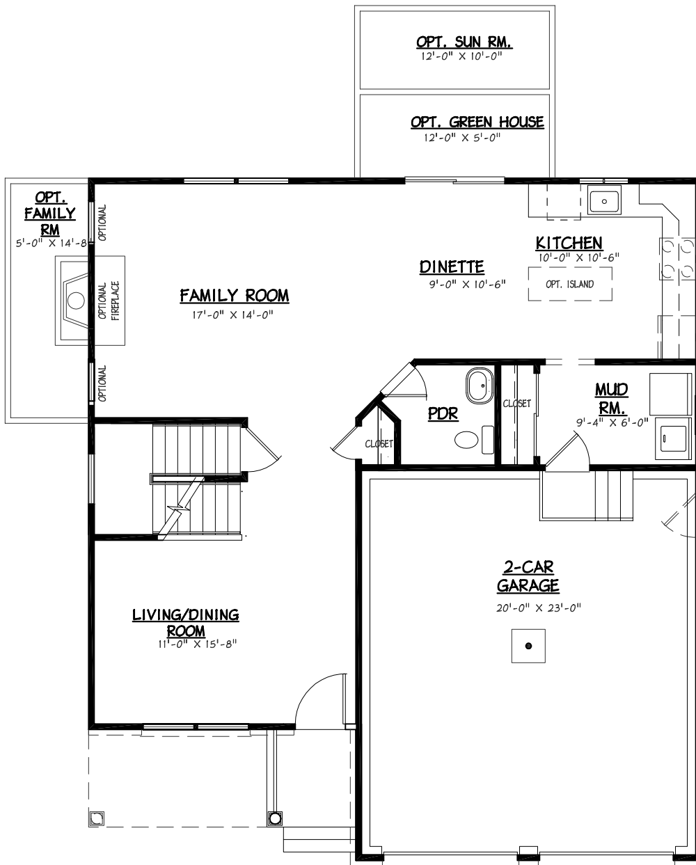
FIRST FLOOR PLAN LIVING AREA 895 SQ. FT.
